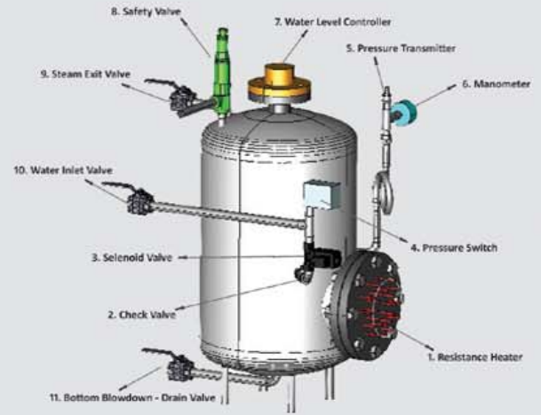
ELK BJ SS LP - Steam Generator Inner Structure and Accessories
